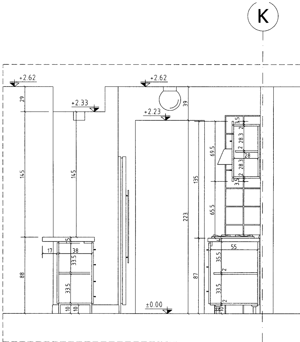
Section 1 28b
